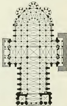
PLAN OF CHARTRES CATHEDRAL
